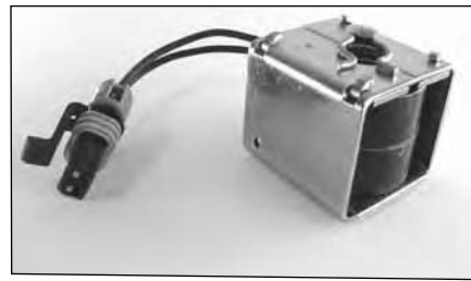
Coil, Solenoid (SV-2 & 4) Order Part #: P-22-02579-00 (Replaces Carrier #: 22-02579-00)
