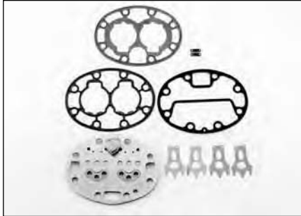
Valve Plate (Canted, Side Bank w/HGBP) Order Part #: P-17-44104-00 (Replaces Carrier #: 17-44104-00)
