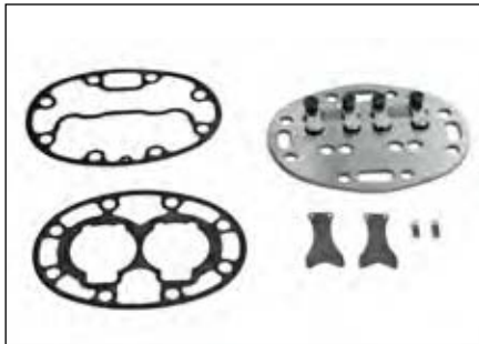
Turn Port Valve Plate TP Center Order Part #: P-17-44742-00 (Replaces Carrier #: 17-44742-00)
