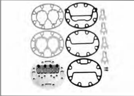
Valve Plate (Canted, Center or Side Bank) Order Part #: P-17-44105-00 (Replaces Carrier #: 17-44105-00)
