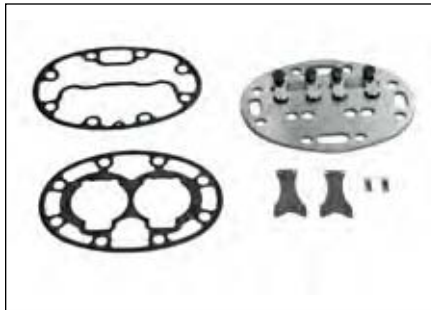
Twin Port Valve Plate TP Side Order Part #: P-17-44744-00 (Replaces Carrier #: 17-44744-00)
